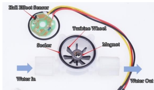
Fig. 6. YF-S201 model transducer
